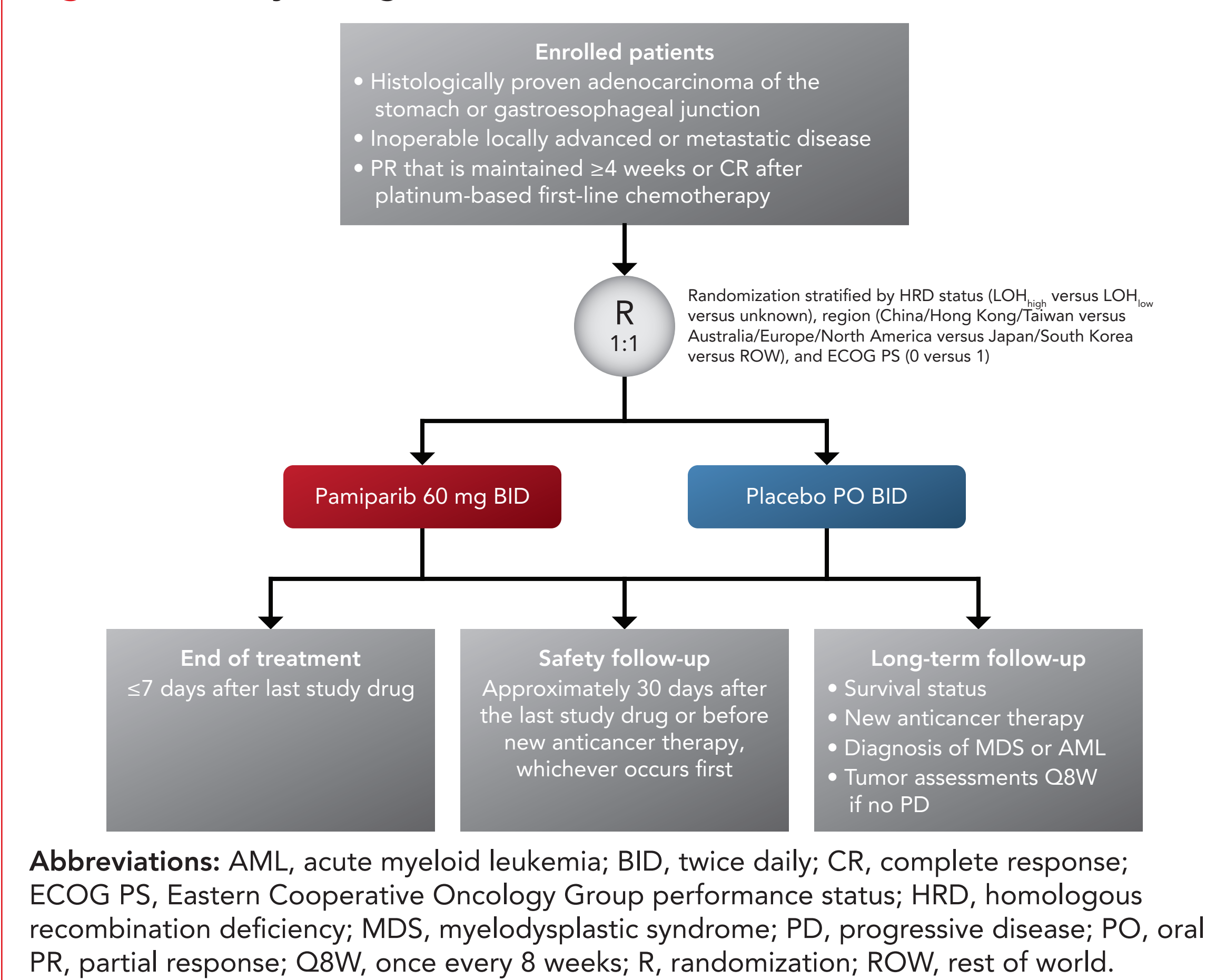
Figure 1: Study Design
